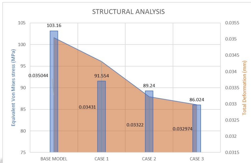
Fig. 5.1 Maximum Total Deformation and Equivalent von Mises Stress
