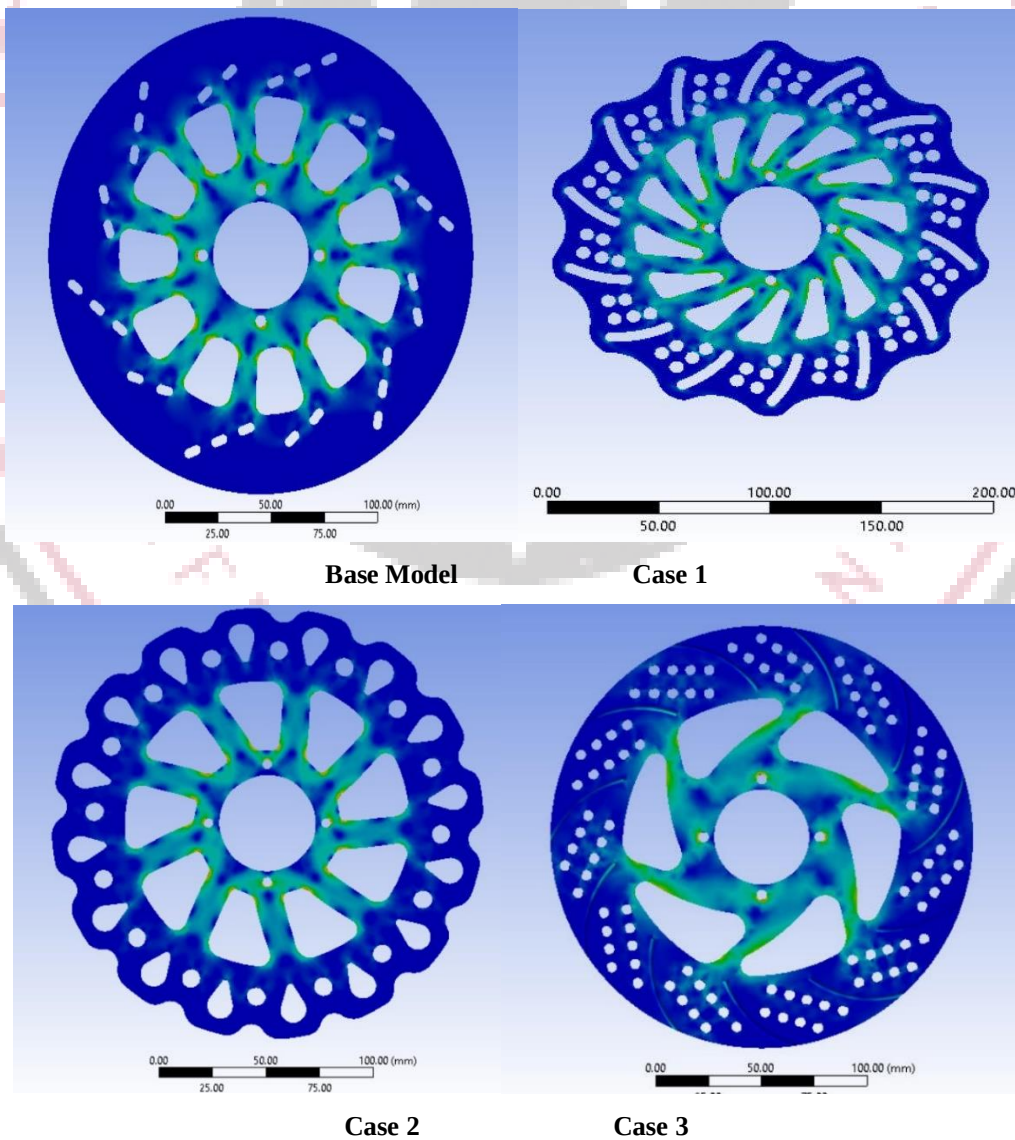
Fig. 4.6 Equivalent stress of all cases
