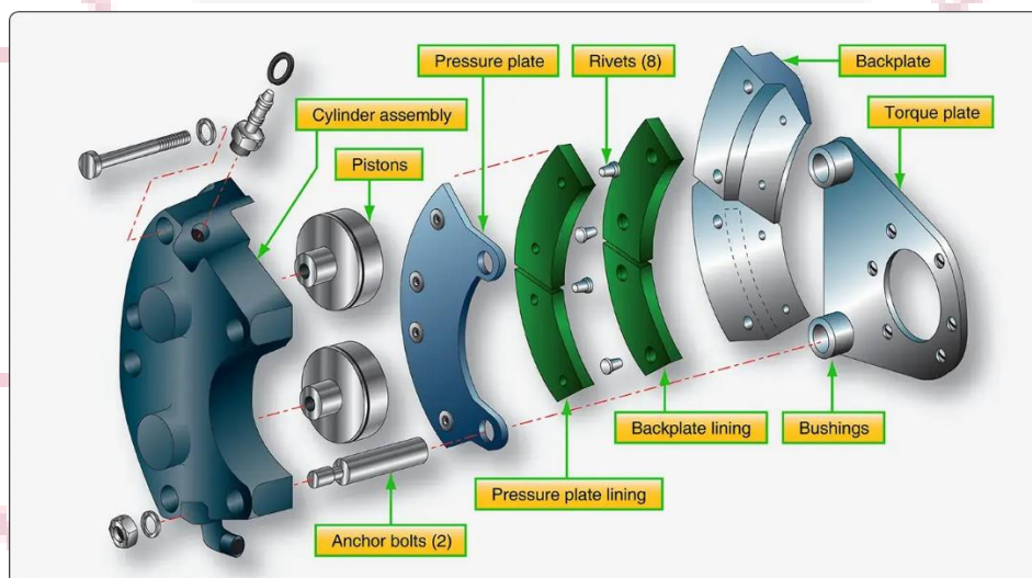
Fig. 1.5 Diagram of Clutch Parts
